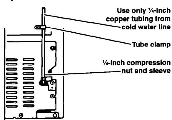
Style #2 valve
